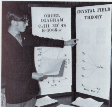
Junior Dennis Trevor—Use of Semi-empirical Parameters in Constructing Orgel Diagrams.—1st Place.
