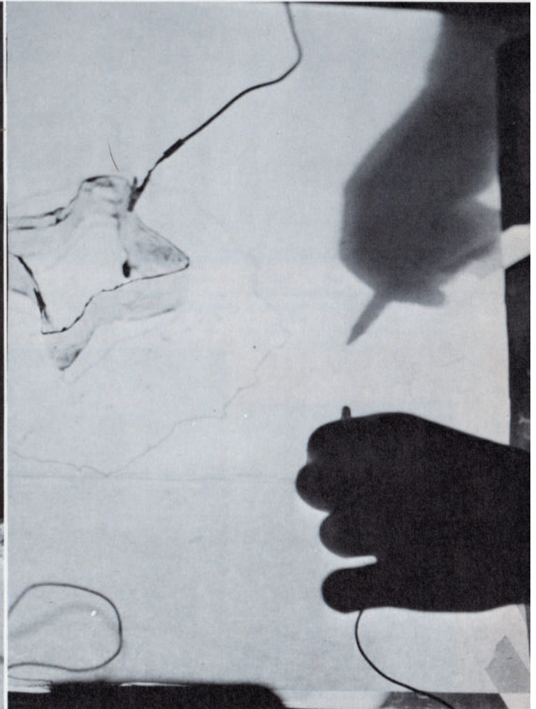
John measures equipotential surfaces in the electric field around a charged conductor.
