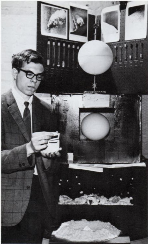
Junior Roger Verbeeren—The Moon, A New Frontier—First Place Award Winner This project belongs to the category of Earth Sciences.
