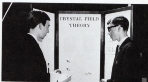
Sophomore Dennis Trevor—Spectra Interpretation of Cobalt Complexes—1st Place. Judge is Terry Renner of DePaul University
