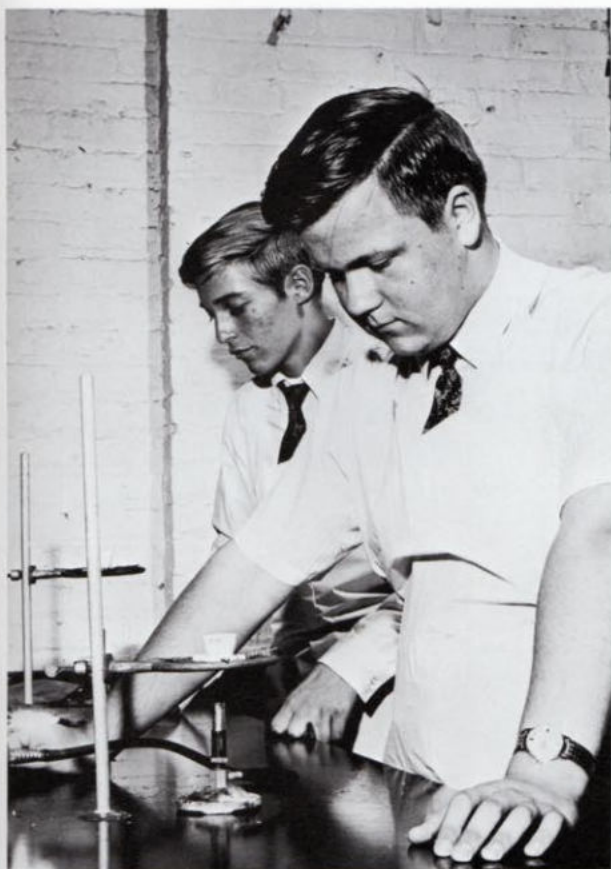
What seems to be a simple experiment often develops into a complex thorough investigation. Chem students, Gerald Schoen and Bob Swiatkowski examine the behavior of solid copper.
