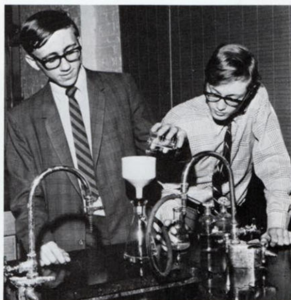
Time is a factor in many chemical reactions. For this reason Dennis Trevor and Gary Kekick use the Buchner filtration.
